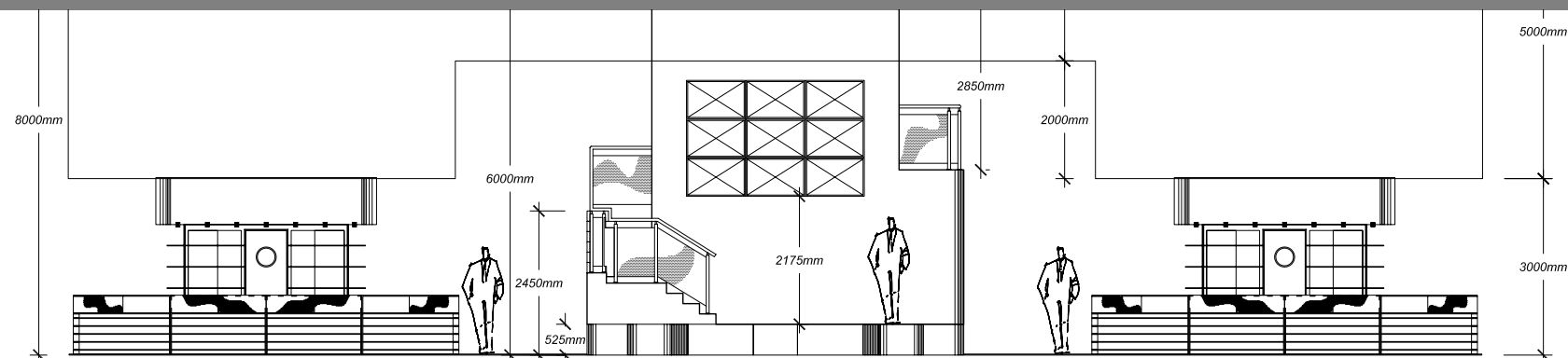
FRONT ELEVATION DRAWN @ 1.75 SCALE
