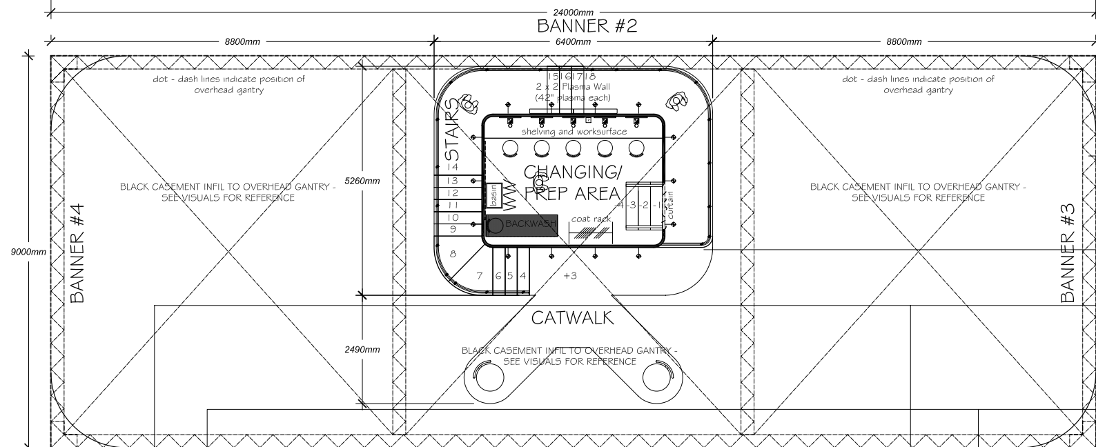
PLAN UPPER DECK DRAWN @ 1.75 SCALE
