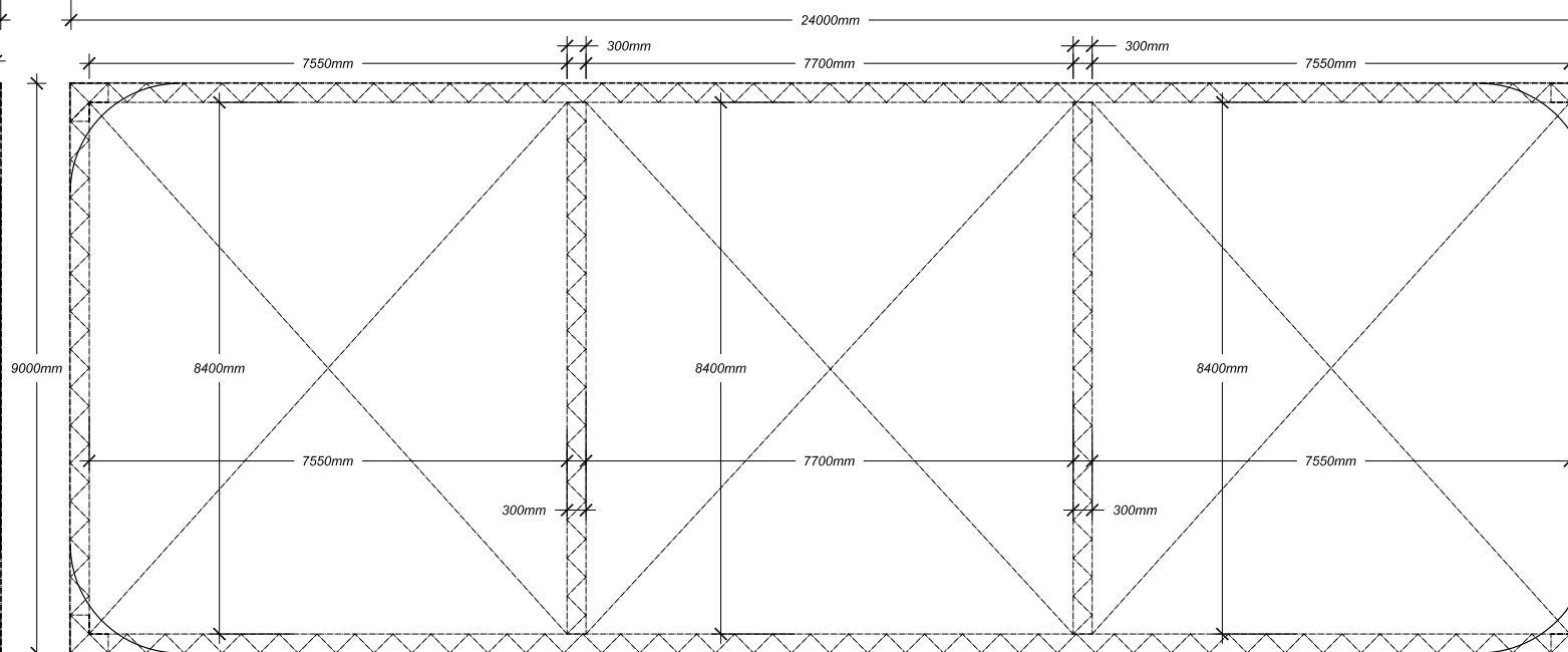
PLAN OF OVERHEAD GANTRY DRAWN @ 1.75 SCALE
