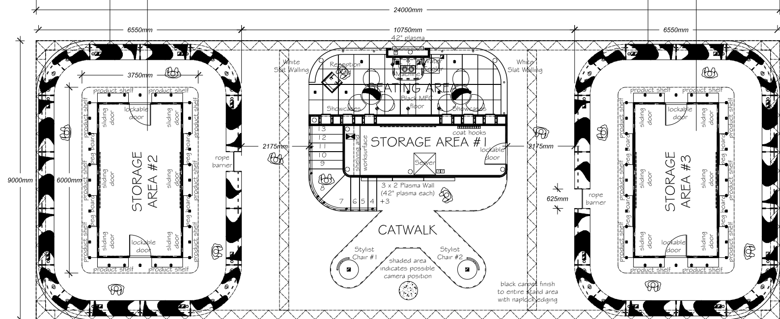
PLAN LOWER DECK DRAWN @ 1.75 SCALE
